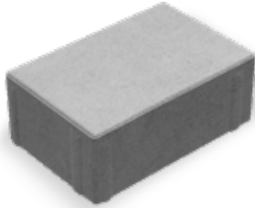
L 211 mm | B 141 mm | H 80 mm
